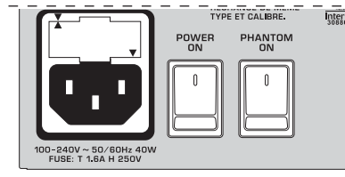
Fig. 2.16: Voltage supply and fuse
